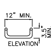
DROP RUNG CATCH BASIN STEP
