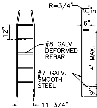
PREFABRICATED LADDER
