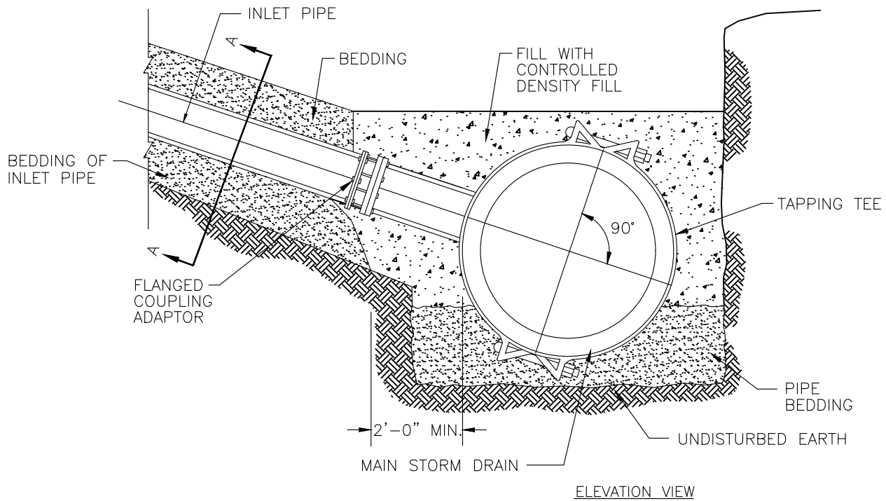
ELEVATION VIEW
