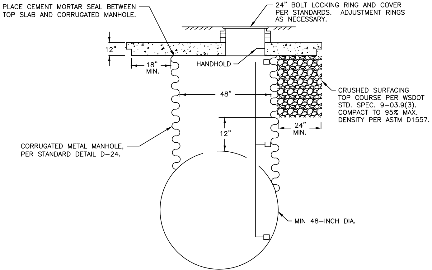
ECCENTRIC SECTION
