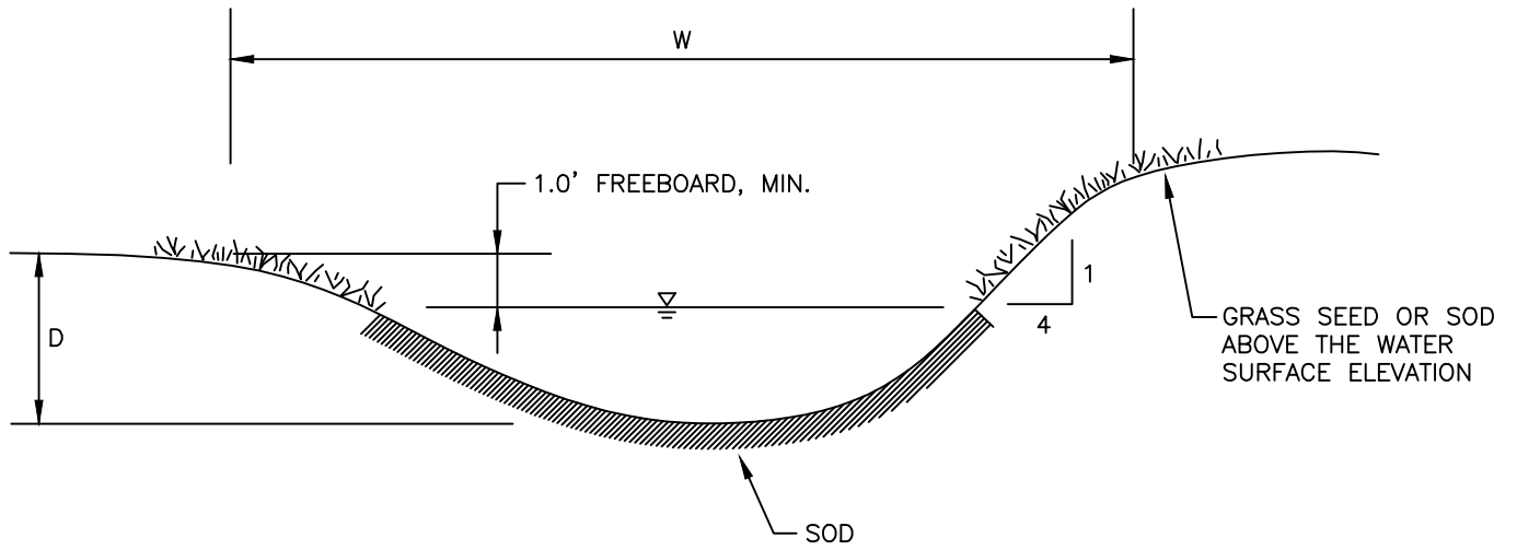
TYPICAL SECTION
