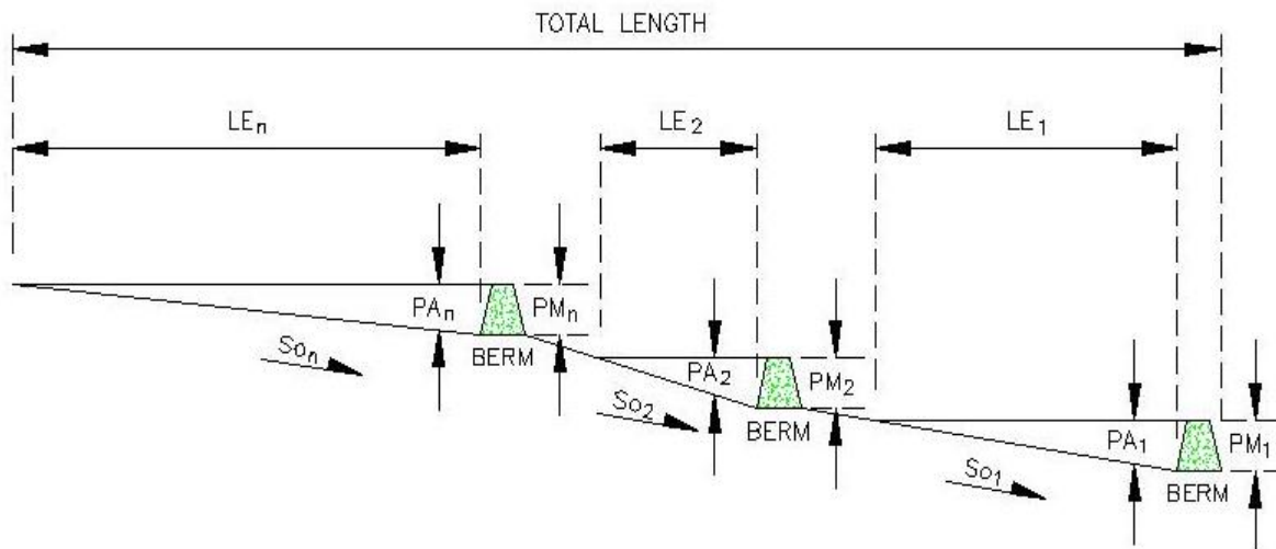
Figure 6.2. Schematic for calculating Bottom Length and Effective Total Depth for bioretention or pervious pavement on slopes where check dams (berms) are used.
