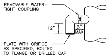
ELBOW DETAIL
