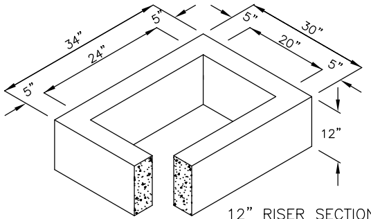
12" RISER SECTION
