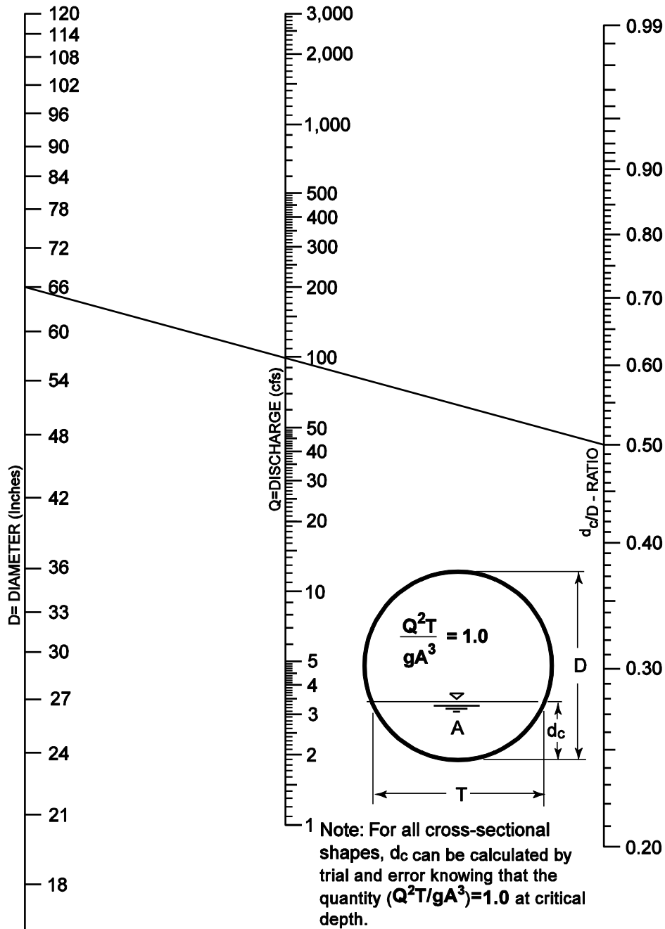
Figure 4. 14 Critical Depth Of Flow For Circular Culverts
