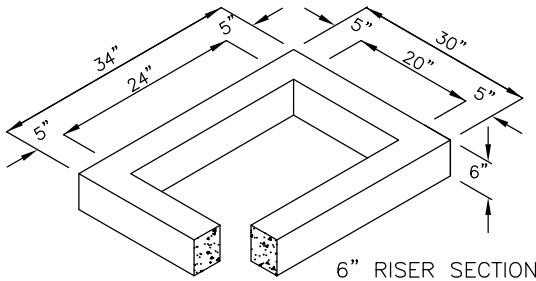
6" RISER SECTION
