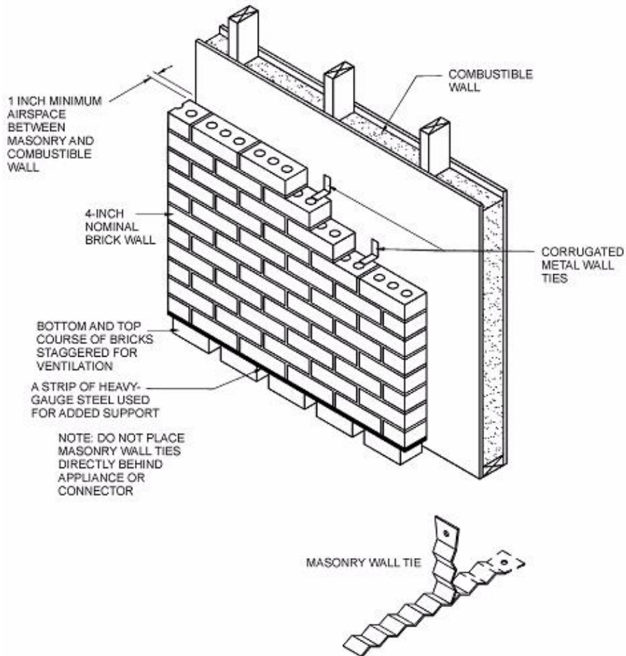
FIGURE G2409.2(2) [308.2(2)] WALL PROTECTOR CLEARANCE REDUCTION SYSTEM
