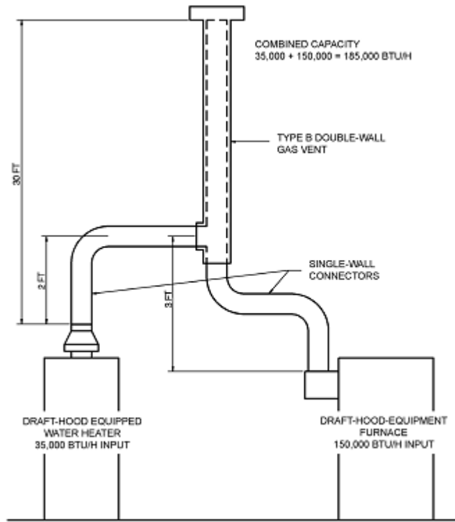
FIGURE B-16 (EXAMPLE 2) SINGLE FAN-ASSISTED APPLIANCE
