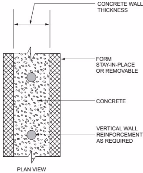
FIGURE R608.3(1) FLAT WALL SYSTEM
