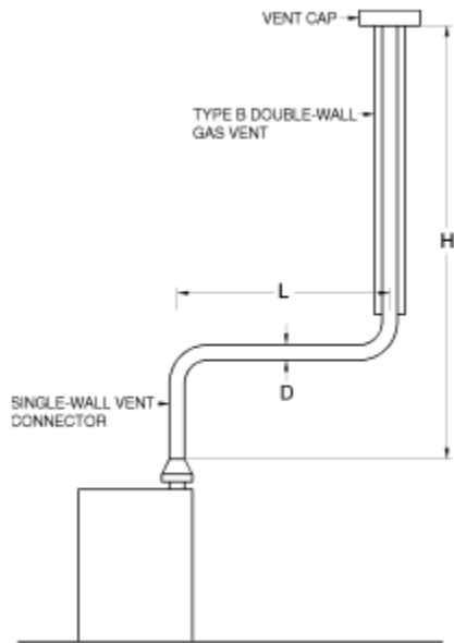
FIGURE B-1 TYPE B DOUBLE-WALL VENT SYSTEM SERVING A SINGLE APPLIANCE WITH A TYPE B DOUBLE-WALL VENT
