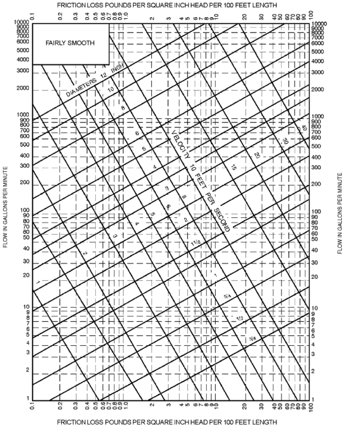
FIGURE AP103.3(4) FRICTION LOSS IN SMOOTH PIPE a (TYPE M, ASTM B 88 COPPER TUBING)
