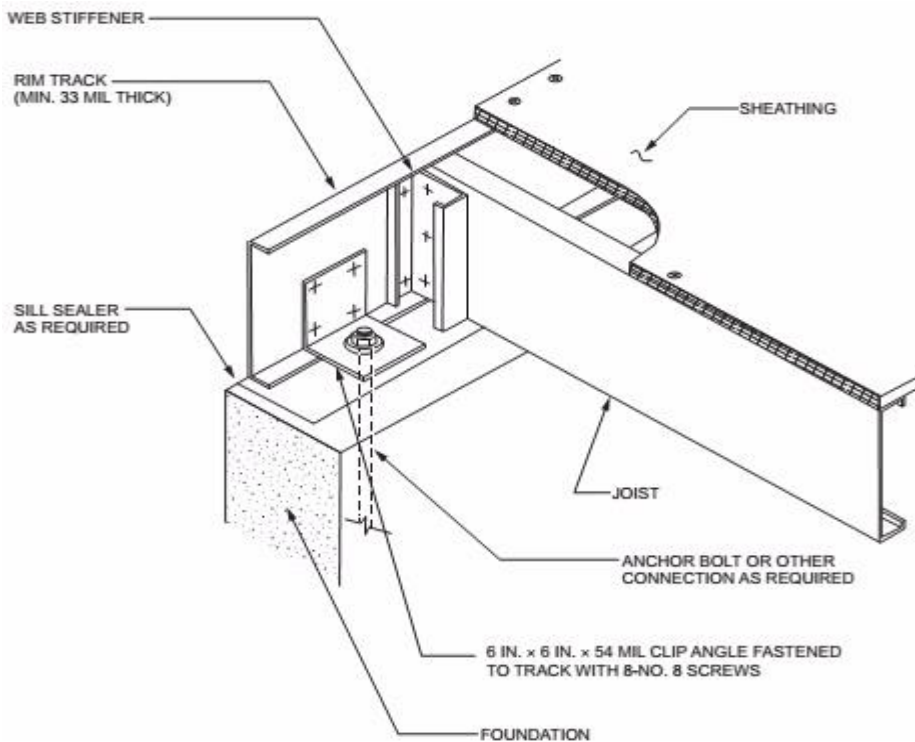
FIGURE R505.3.1(2) FLOOR TO WOOD SILL CONNECTION
