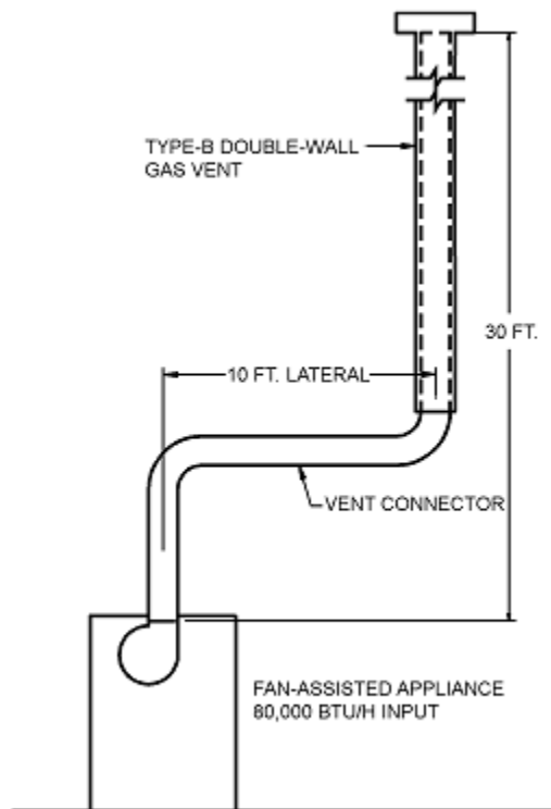
FIGURE B-15 (EXAMPLE 1) SINGLE DRAFT-HOOD-EQUIPPED APPLIANCE
