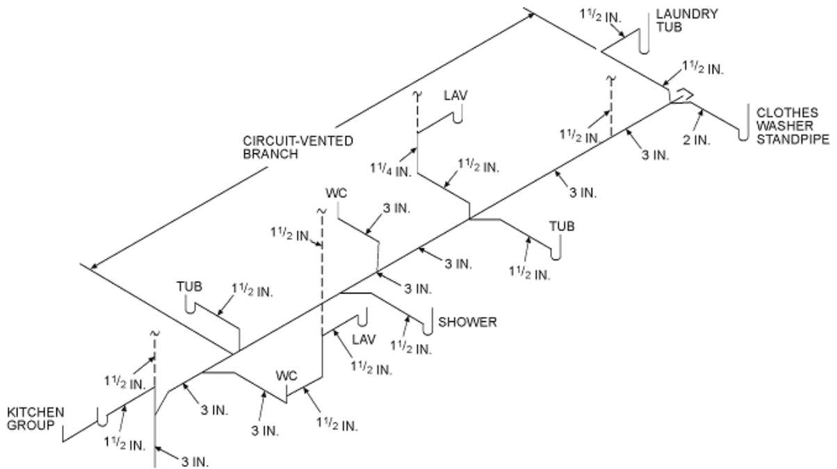
FIGURE N6 WASTE STACK VENTING
