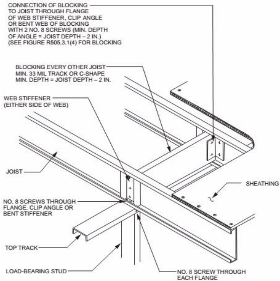
FIGURE R505.3.1(7) CONTINUOUS SPAN JOIST SUPPORTED ON INTERIOR LOAD-BEARING WALL
