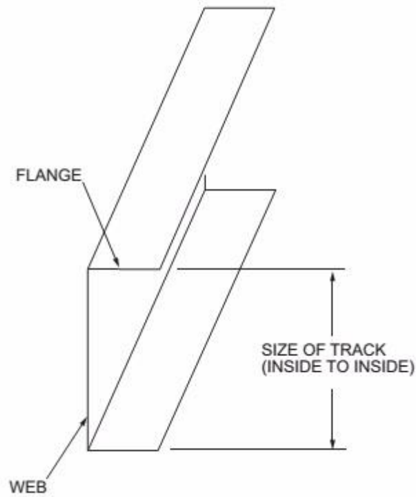
FIGURE R804.2.3(1) C-SHAPED SECTION
