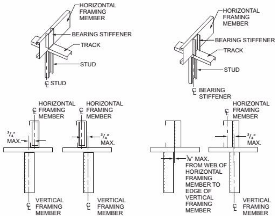
FIGURE R603.1.2 IN-LINE FRAMING
