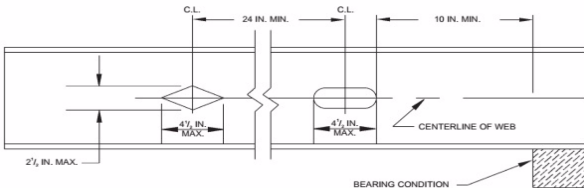
FIGURE R505.2.6.1 FLOOR JOIST WEB HOLES
