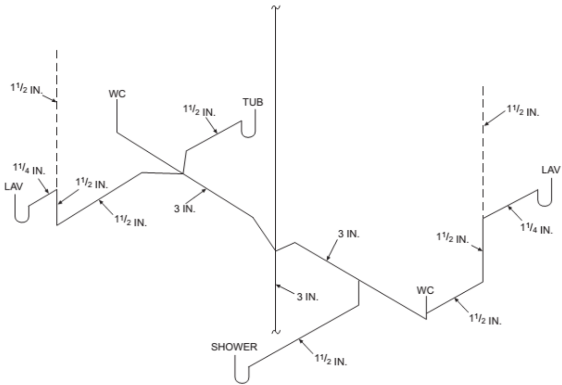
B. HORIZONTAL WET VENTING
