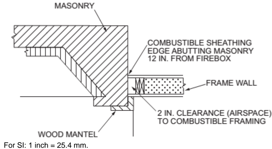
FIGURE R1001.11 CLEARANCE FROM COMBUSTIBLES
