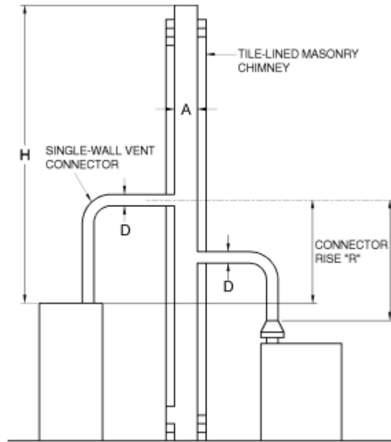
FIGURE B-8 MASONRY CHIMNEY SERVING TWO OR MORE APPLIANCES WITH TYPE B DOUBLE-WALL VENT CONNECTOR
