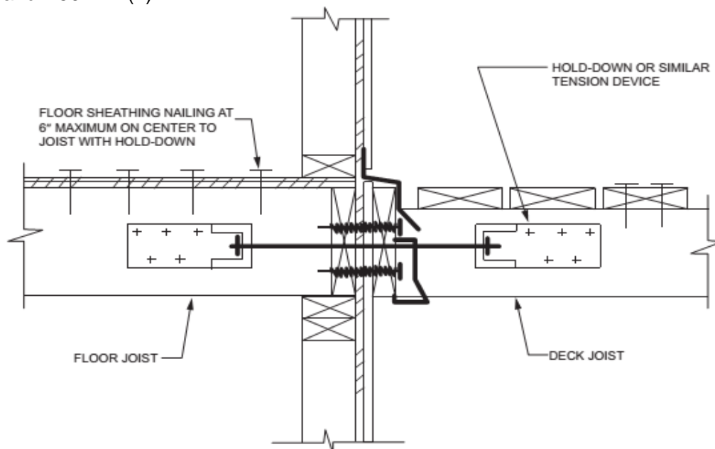
FIGURE 507.2.3(1) DECK ATTACHMENT FOR LATERAL LOADS
