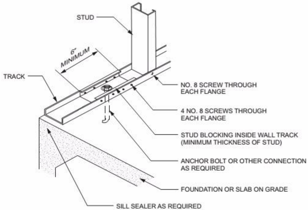
FIGURE R603.3.1(1) WALL TO FLOOR CONNECTION
