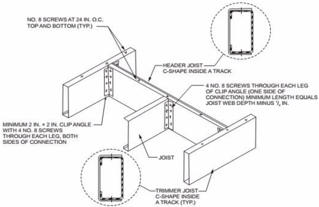
FIGURE R505.3.8(3) COLD-FORMED STEEL FLOOR CONSTRUCTION: FLOOR HEADER TO TRIMMER CONNECTION—6-FOOT OPENING
