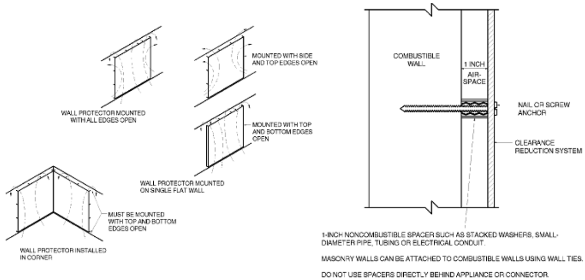
FIGURE G2409.2(2) [308.2(2)] WALL PROTECTOR CLEARANCE REDUCTION SYSTEM
