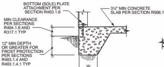
1 MONOLITHIC SLAB-ON-GROUND WITH TURNED-DOWN FOOTING
