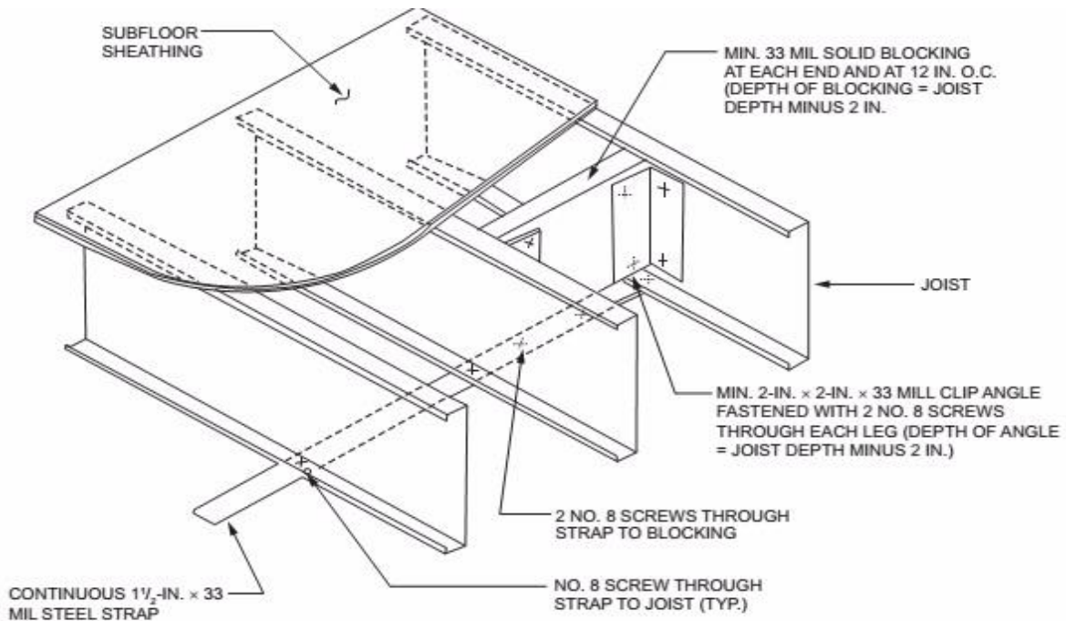
FIGURE R505.3.3.2(1) JOIST BLOCKING (SOLID)
