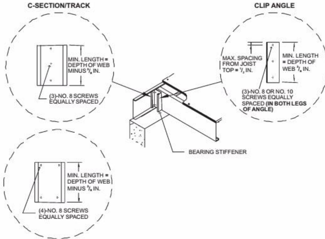
FIGURE R505.3.4(1) BEARING STIFFENERS UNDER JAMB STUDS
