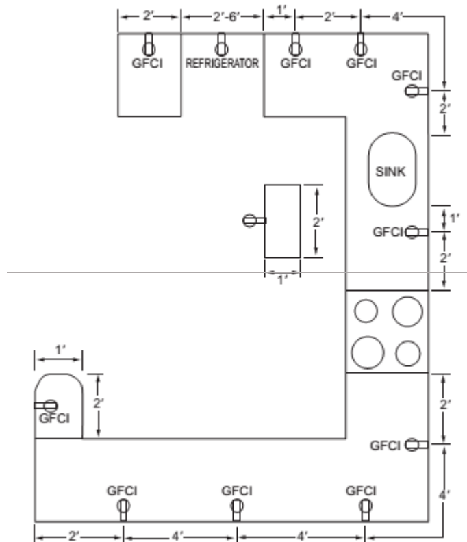
FIGURE E3901.4 COUNTERTOP RECEPTACLES
